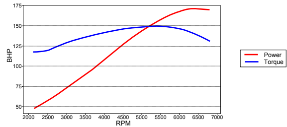
Typical Zetec Blacktop 2.0 Long Throttle Body Kit Power Graph
